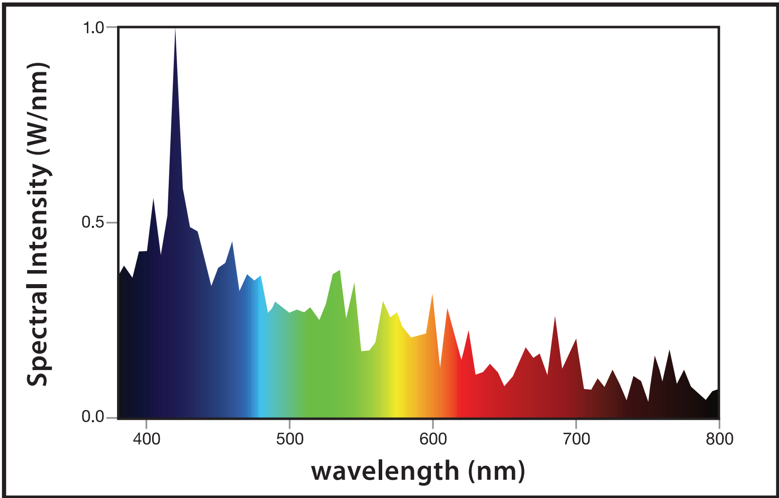
Ultra Sun 1000 Watt - 10,000°K MH Lamp - Spectral Intensity Graph
